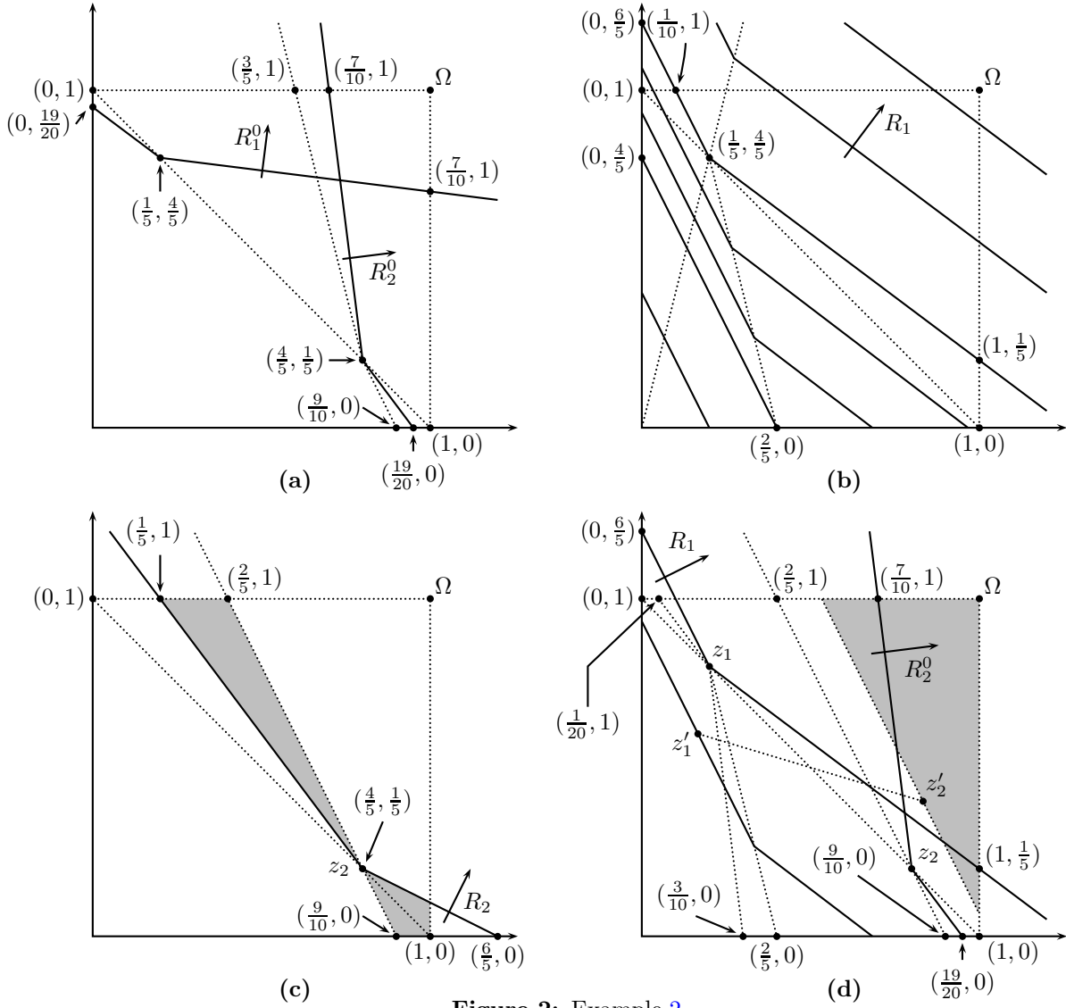
Figure 2: Example 2.
